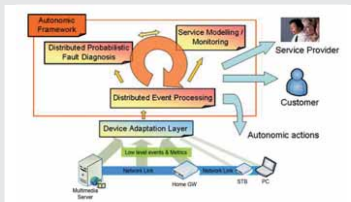
Figure 2: Autonomic loops
