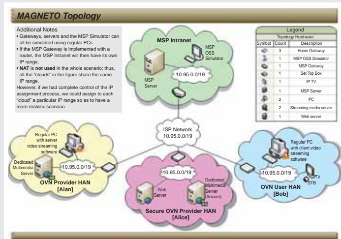
Figure 1: Magneto topology
